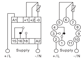
RTD/Thermistor (3-wire)
